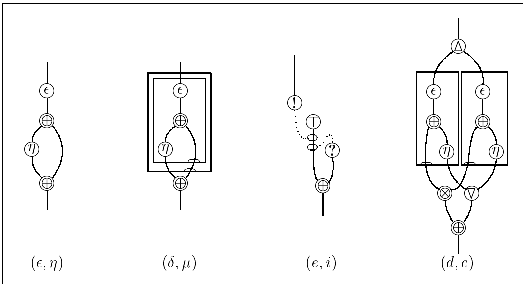
Fig. 16. Nets needed to show some transformations are linear
