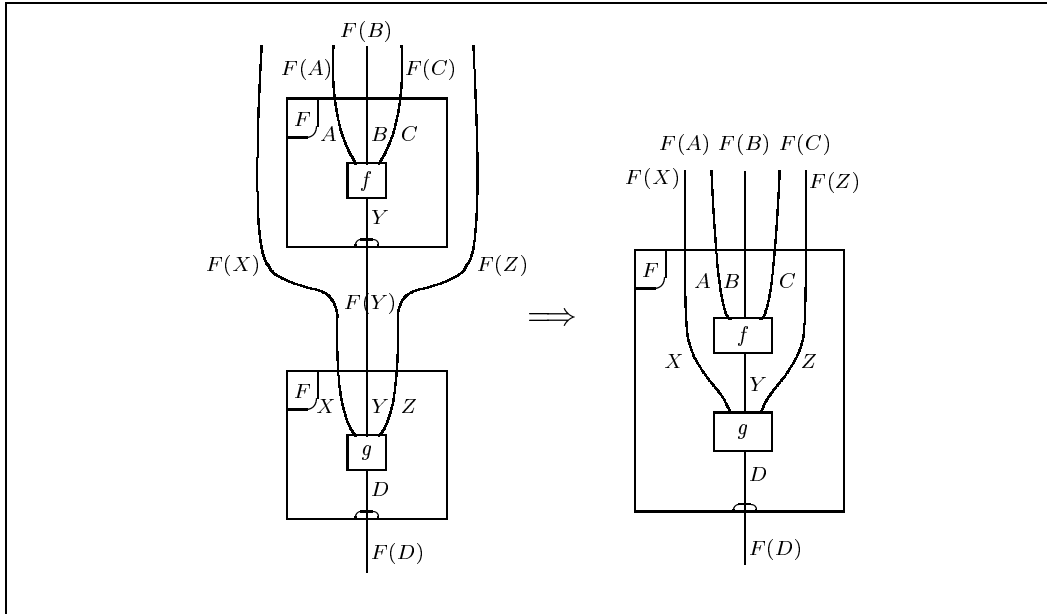
Fig. 4. Box-eats-box rule
