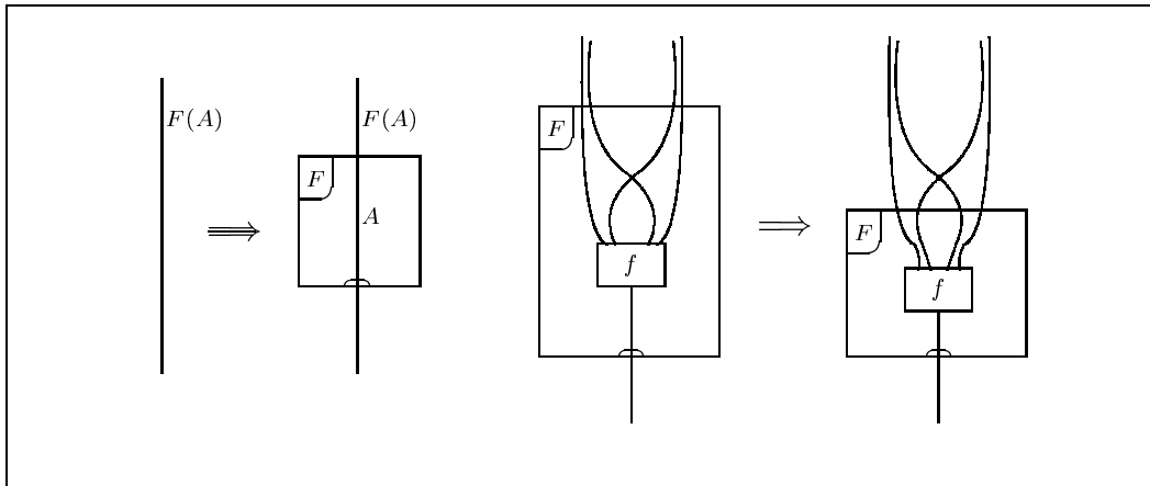
Fig. 5. Expansion and twist rules
