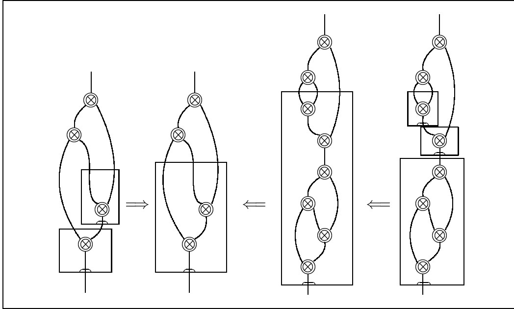
Fig. 6. Functor boxes are monoidal—equation (2)
