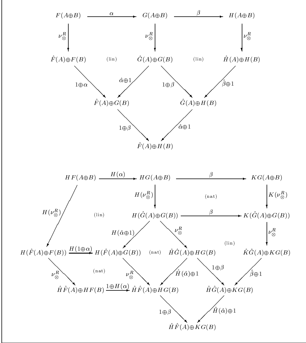
Fig. 2. Coherence for \alpha; \beta — vertical and horizontal
