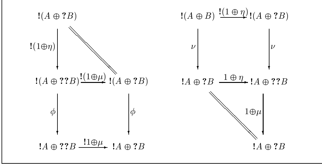
Fig. 14. Diagrams verifying the bijection \phi \leftrightarrow \nu
