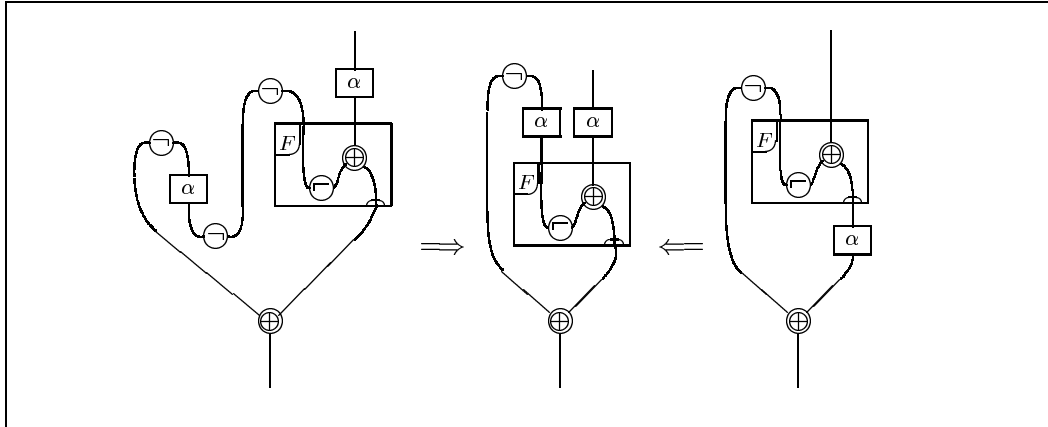
Fig. 12. Validity of equation (11)
