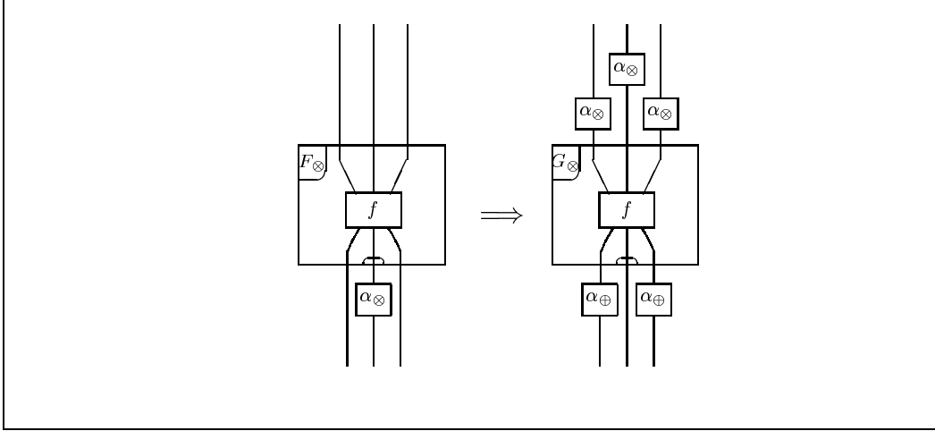
Fig. 9. Rewrite rule for linear transformations
