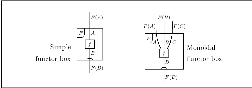
Fig. 3. Functor boxes
