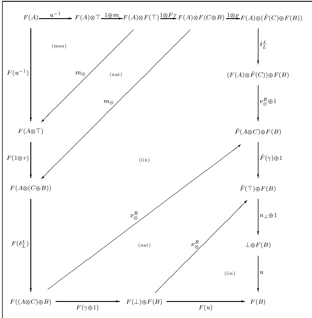
Fig. A.1. Linear F preserves nuclear f
