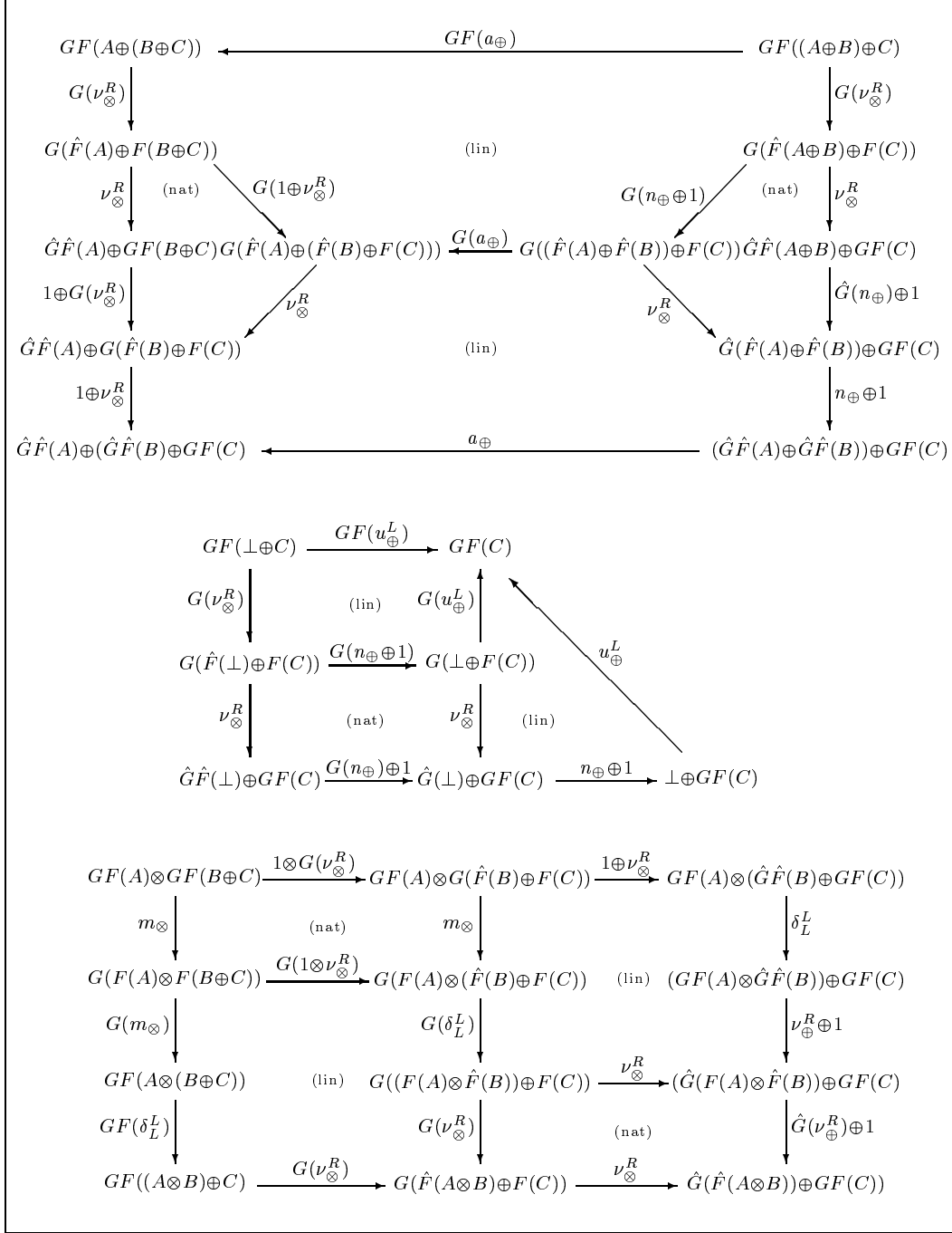
Fig. 1. Coherence for F; G
