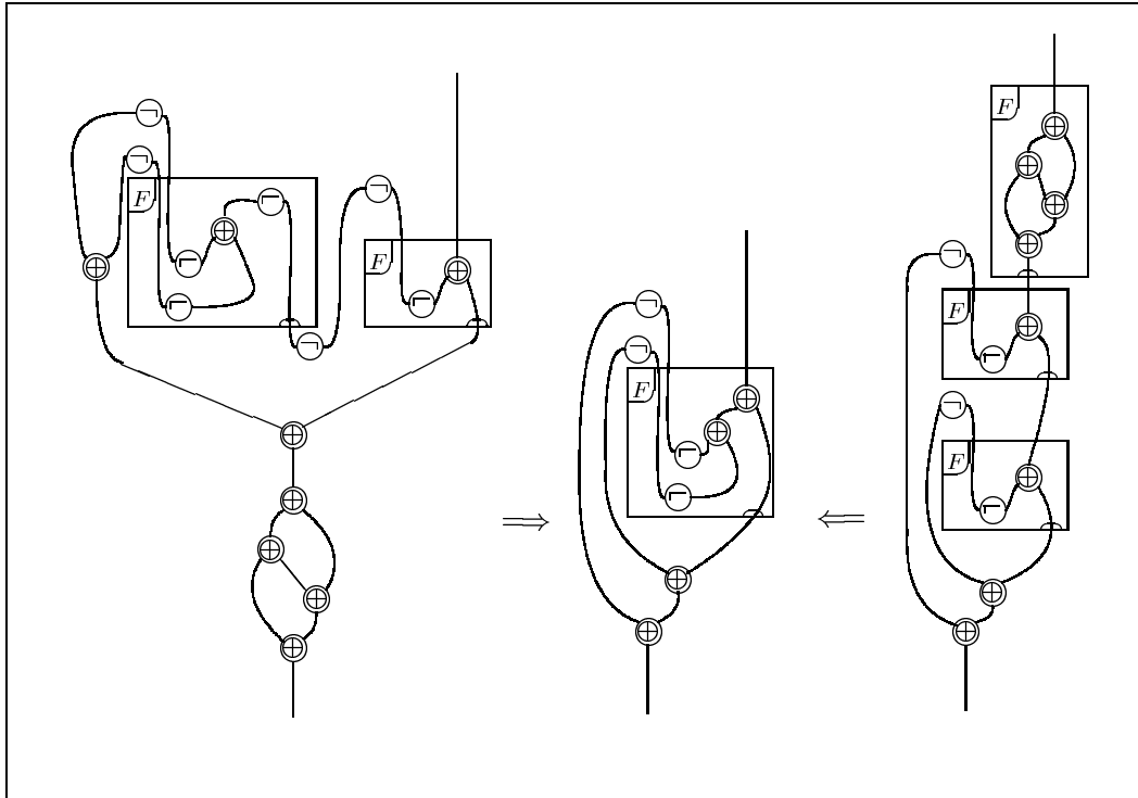
Fig. 10. Validity of equation (5)
