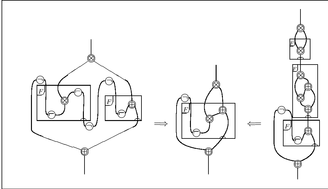
Fig. 11. Validity of equation (7)
