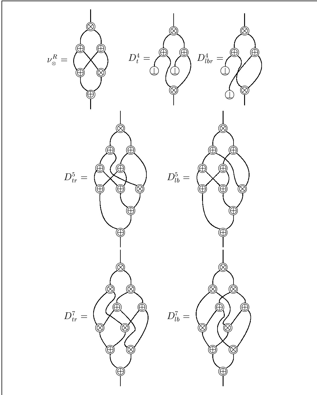
Fig. 13. Nets needed to show coherence for \otimes
