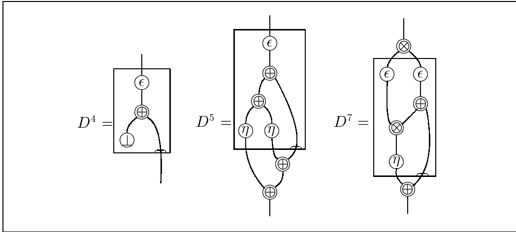
Fig. 15. Nets needed to show \mathbb{!} is linear
